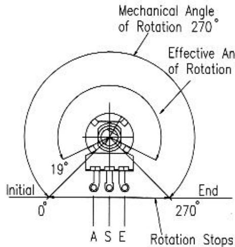
SPINDLE END VIEW
