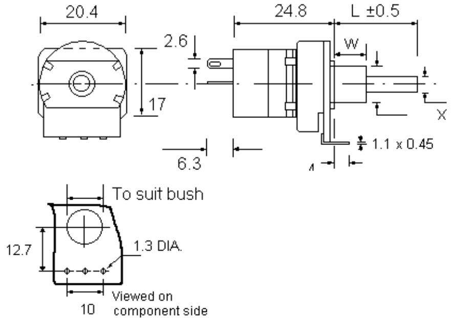
SPINDLE END VIEW
