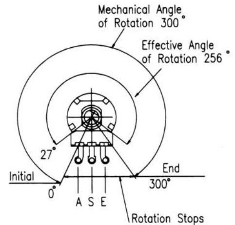
Total mechanical and effective electrical angles of rotation of potentiometers
