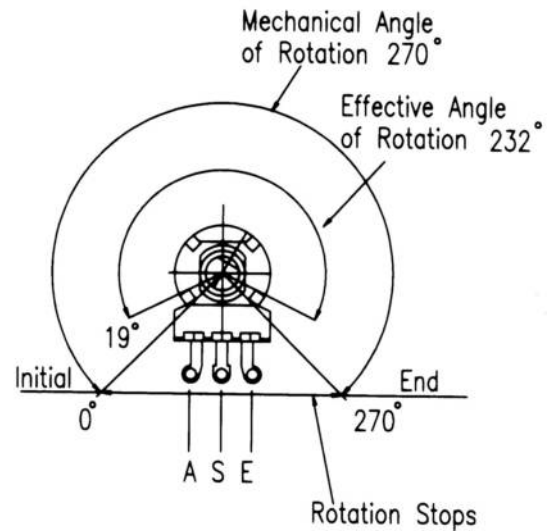
Total mechanical and effective electrical angles of rotation of potentiometers without rotary switch
