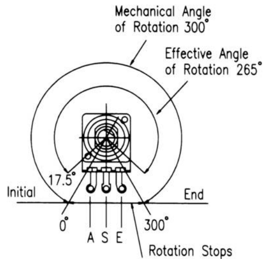
SPINDLE END VIEW
