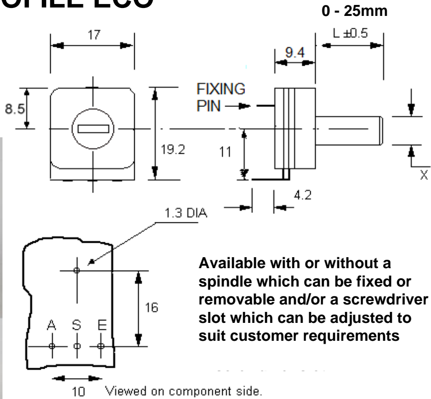
SPINDLE END VIEW
