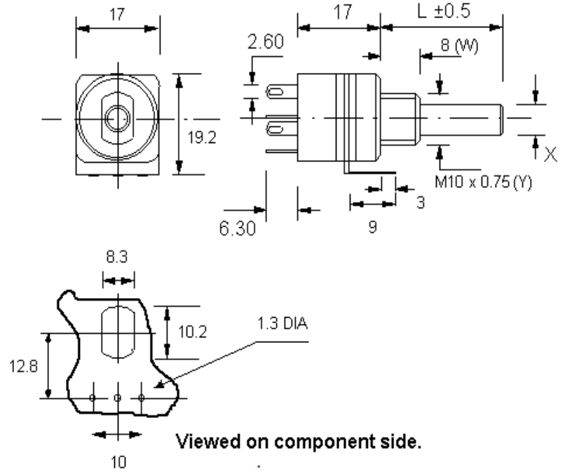
SWITCH ORDINARY WIRING (OW) TERMINALS.
