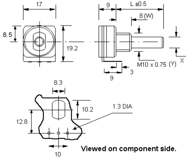
SPINDLE END VIEW
