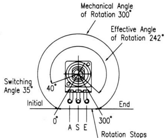
SPINDLE END VIEW
