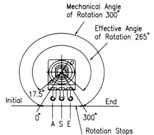
Total mechanical and effective electrical angles of rotation of potentiometers
