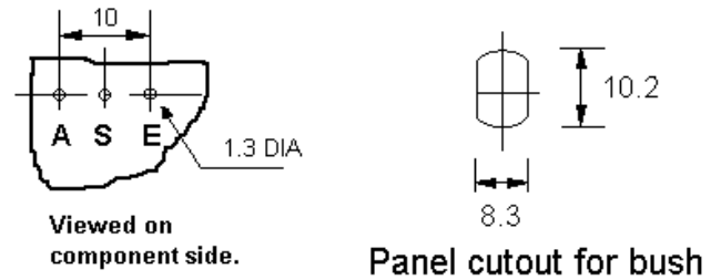
POTENTIOMETER with PRINTED CIRCUIT (PC) TERMINALS.
