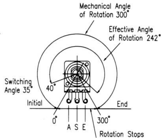
SPINDLE END VIEW
