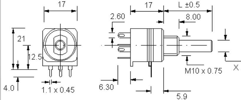
POTENTIOMETER with PRINTED CIRCUIT (PC) TERMINALS.
