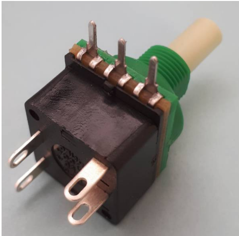
POTENTIOMETER with PRINTED CIRCUIT (PC) TERMINALS.
