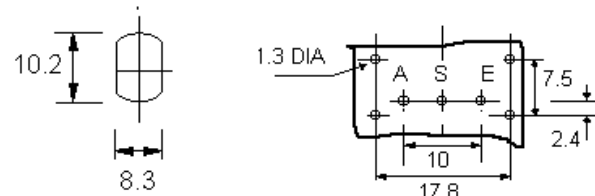
Panel cutout for bush
