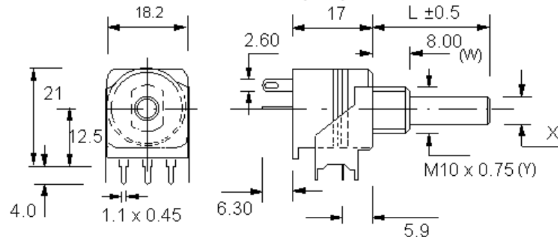
POTENTIOMETER PRINTED CIRCUIT (PC) TERMINALS.
