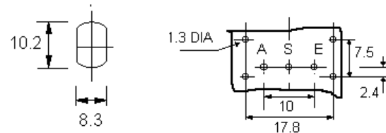
Panel cutout for bush
