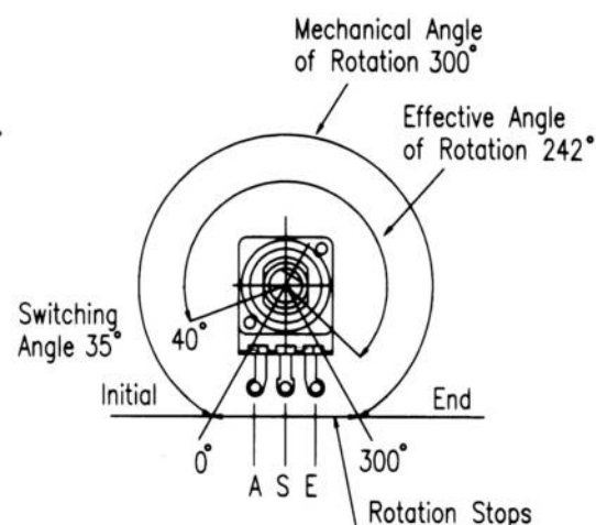
SPINDLE END VIEW
