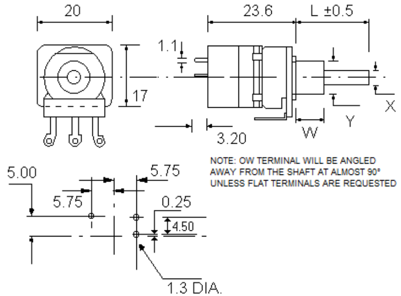
SPINDLE END VIEW
