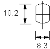
Panel cutout for bush
