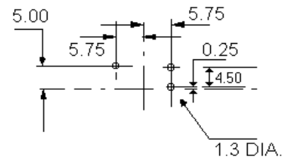
Viewed on component side
