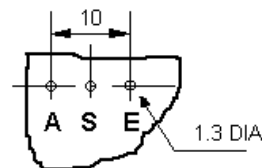
POTENTIOMETER with PRINTED CIRCUIT (PC) TERMINALS.
