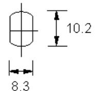
POTENTIOMETER with PRINTED CIRCUIT (PC) TERMINALS.
